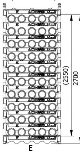
5 SYSTEMS STACKED (50 JOINTS)
